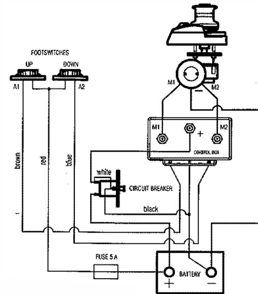
WIRING DIAGRAM - 3 TERMINALS ELECTRIC MOTOR
